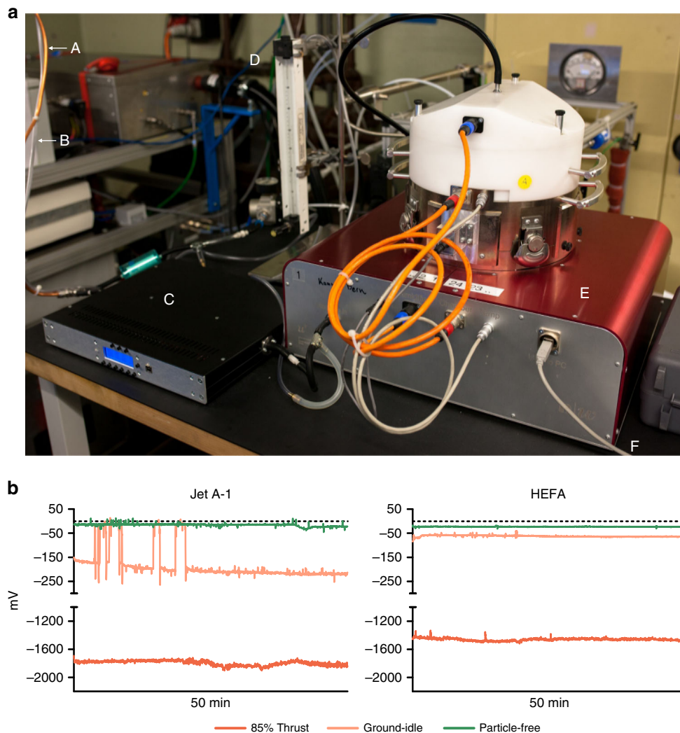
Fig. 2 Aerosol exposure setup and particle deposition. a NACIVT deposition chamber setup for jet turbine aerosol exposure. A = Exhaust line; B = CO 2 line; C = low-flow thermodenuder; D = rotameter for regulation of CO 2 flow into the chamber (5%); E = NACIVT chamber; and F = USB connection to computer for online data collection. b Successful deposition of particles on cell cultures. Electrometer data collected within the deposition chamber show distinct precipitation voltage patterns for varying engine thrust levels and fuel types
