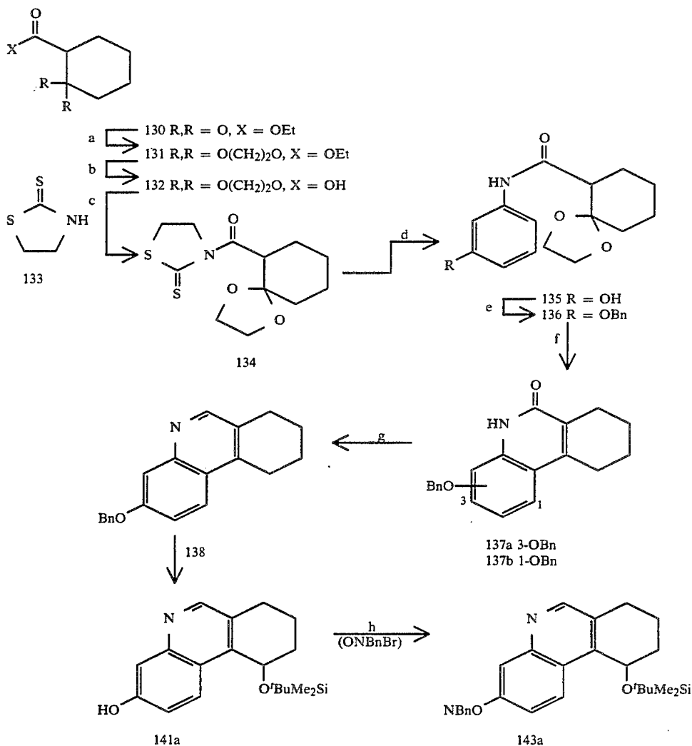
Scheme XVII
