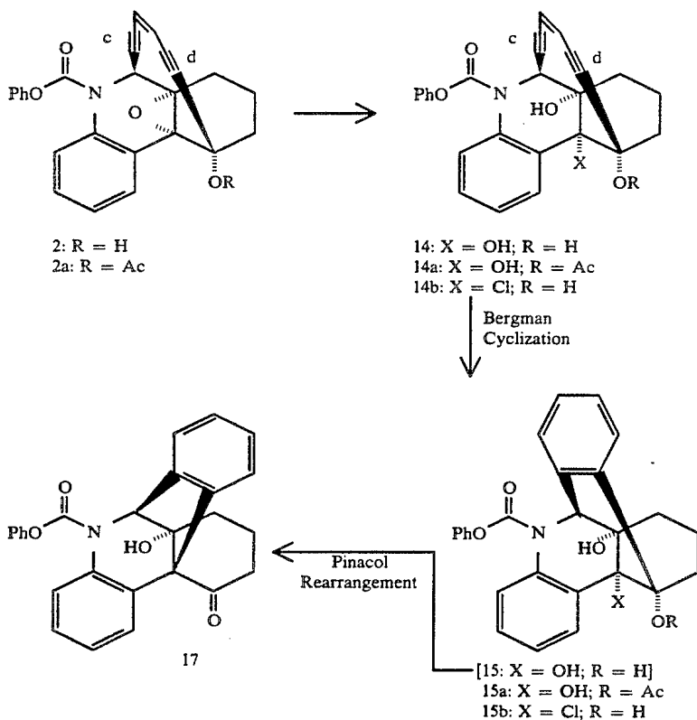
Scheme V
