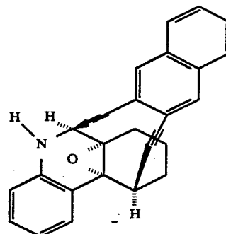
Compound 87a
