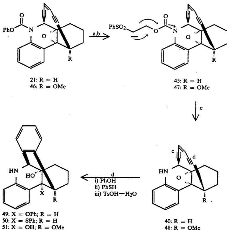
Scheme VIII
