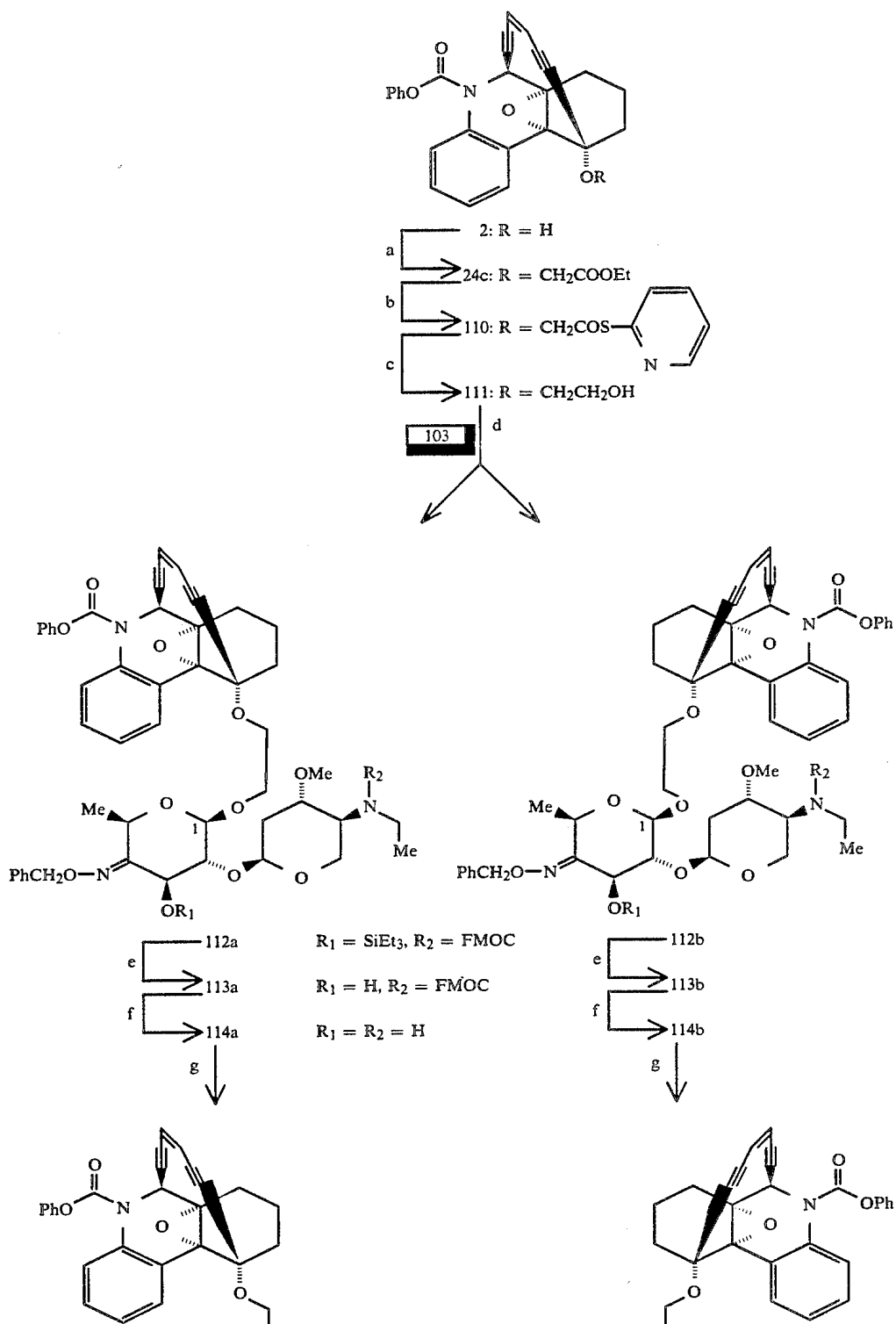
Scheme XIV
