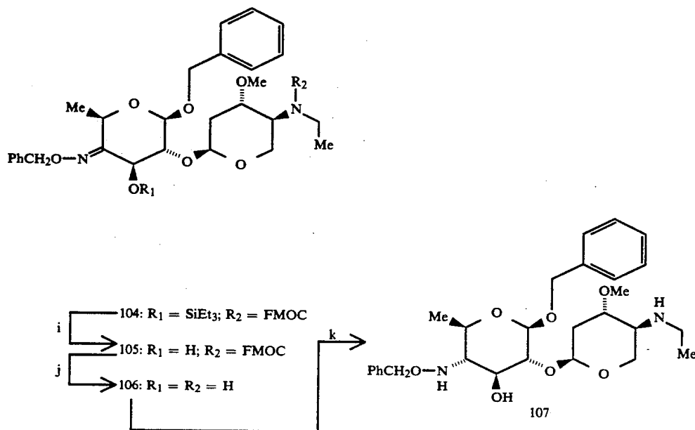
Scheme XIII
