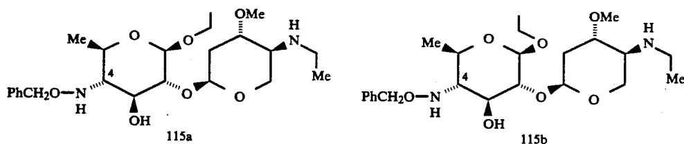
Scheme XIV
