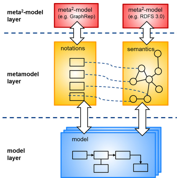
Fig. 4.3. Semantic metamodelling.
