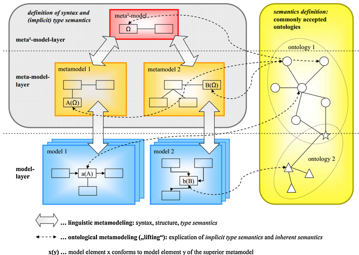
Fig. 4.2. Metamodels for human-interpretable and machine-interpretable models [52].
