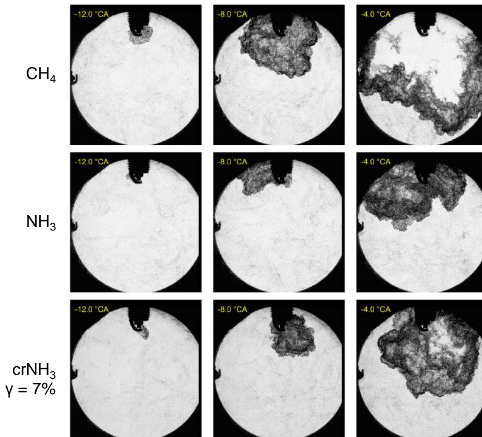
Figure 4: Schlieren images of CH 4 (top row) NH 3 (middle row) and partially cracked NH 3 ( \gamma = 7\% , bottom row) at \lambda = 1.25 , n = 600 \text{ min}^{-1} , p_c = 70 \text{ bar} , T_{in}(\text{CH}_4) = 323 \text{ K} , T_{in}(\text{NH}_3) = T_{in}(\text{crNH}_3) = 373 \text{ K}
