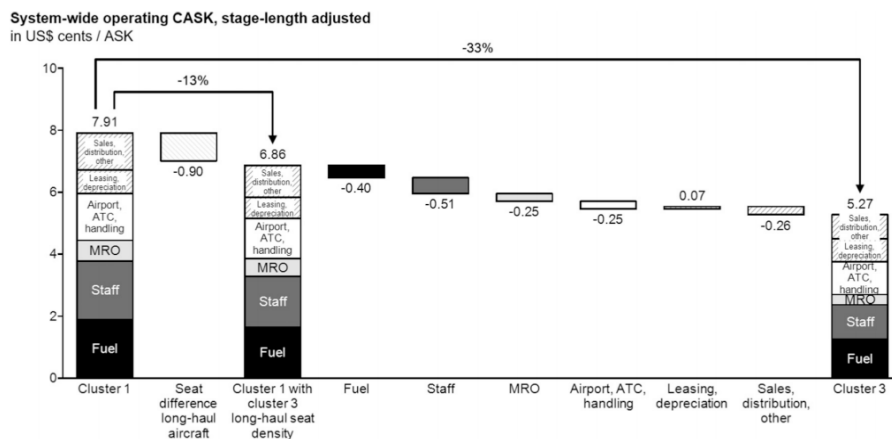
Fig. 1. Differences in operating costs between airlines from two derived clusters by cost items. Source: (Soyk et al. 2017).
