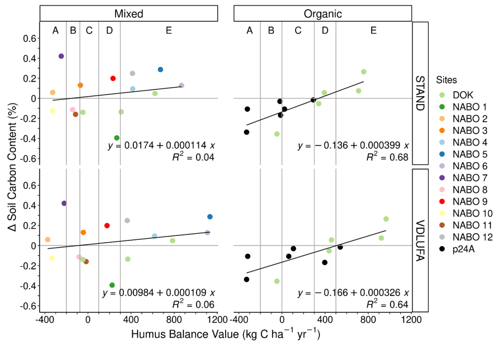
FIGURE 3 Correlation between humus balance value determined by the STAND (top) and VDLUFA (bottom) methods and observed change in soil carbon content of short-term observations with mixed (left) and organic (right) fertilization. The humus supply groups are labelled A–E at the top of each graph and represent the very low (A), low (B), balanced (C), high (D) and very high (E) humus supply evaluations. Standard errors for changes in soil carbon content for single crop rotations ranged from 0.023% to 0.22% for the DOK trial (mean 0.13%); 0.0084% to 0.063% for NABO sites (mean 0.026%) and 0.034% to 0.15% (mean 0.084%) for the p24A experiment. Because standard errors could not be calculated for every rotation (in some cases, only one composite sample was available), we do not show error bars.
