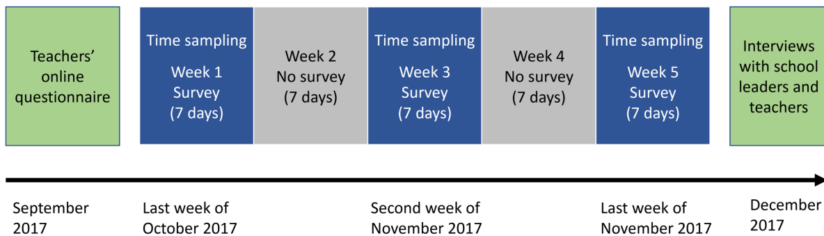
Figure 1. Research design
