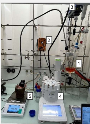
Figure 3: experimental setup. 1: reactor; 2: dosing pump; 3: Stirrer; 4: automated sampler; 5: scale for dosing pump
