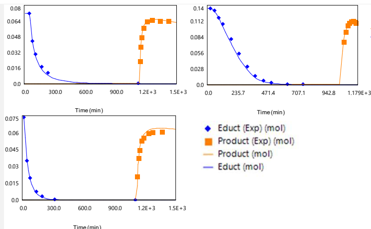
Figure 6: comparison of selected experimental data (points) with model prediction (solid lines) of educt 1 in blue and product 2 in orange.
