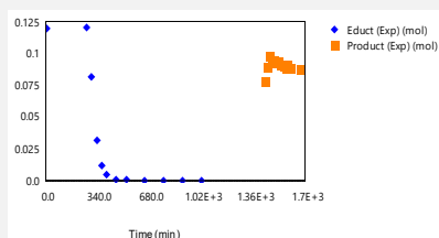
Figure 4: example of experimental HPLC data acquired.
