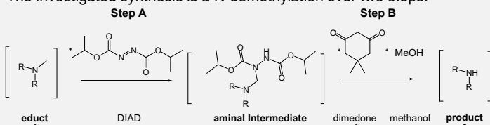
Figure 2: synthesis scheme for the investigated synthesis steps.
