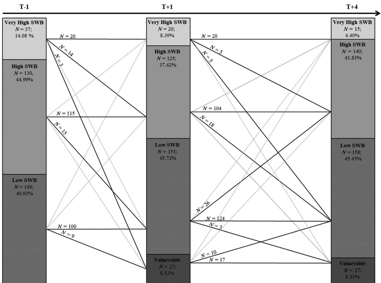
Figure 2 Profile Transition Between SWB Profiles Across T - 1, T + 1, and T + 4
