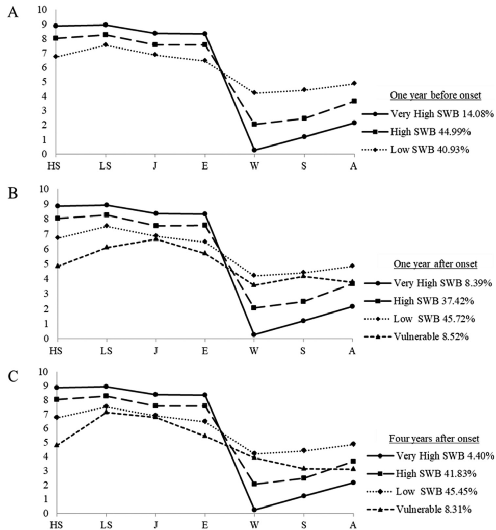
Figure 1 Profiles of SWB at T - 1 , T + 1 , and T + 4
